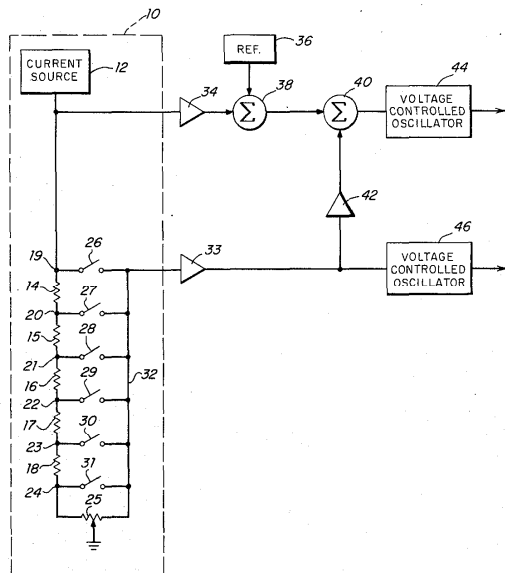
Figure 3 1974 ARP dual keyboard circuit
