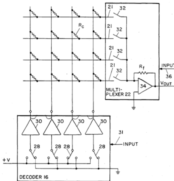
Figure 12 Grounding and virtual ground sensor isolation
