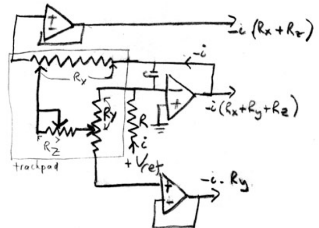
Figure 8 Concurrent Sensing for the Slab
