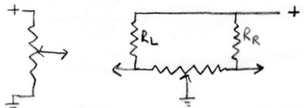
Figure 1. Potential divider (left), and Grounded wiper (right)
