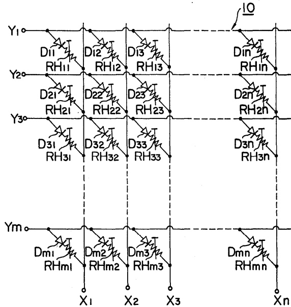
Figure 11 Diode isolated variable resistor array.
