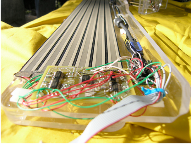
Figure 5: Stringless Cello Position and Pressure Strips
