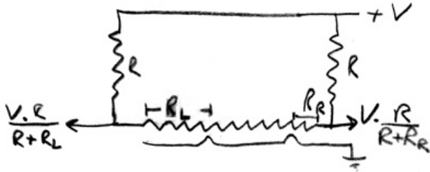
Figure 2 Sensing 2 points with Membrane potentiometers
